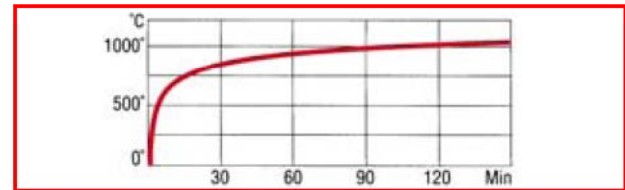
Tested according to the internationally standardised temperature curve (ISO 834).
