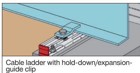
Cable ladders
