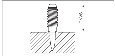
h_{NVS} = 17.0 - 20.0 \text{ mm}
