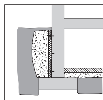
Insulation of basement perimeter/foundation walls
